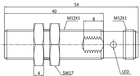
Fig. 7 Inductive sensor with M12 connector (non-flush)
