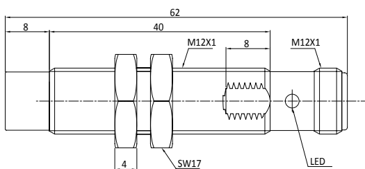
Fig. 7 Inductive sensor with M12 connector (non-flush)
