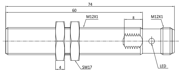
Fig. 8 Inductive sensor with M12 connector (non-flush)
