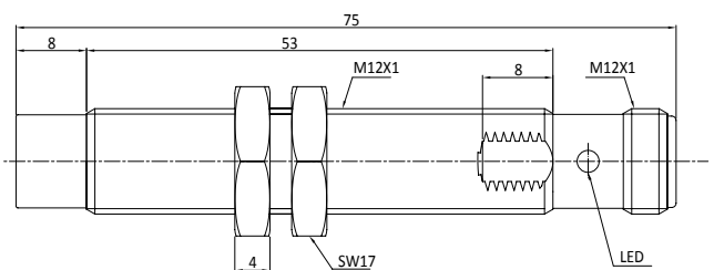
Fig. 8 Inductive sensor with M12 connector (non-flush)
