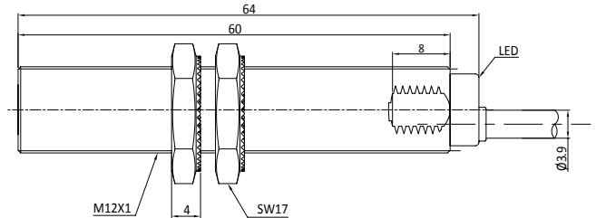
Fig. 4 Inductive sensor with cable (non-flush)
