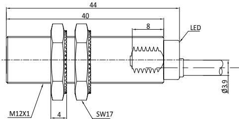
Fig. 3 Inductive sensor with cable (non-flush)
